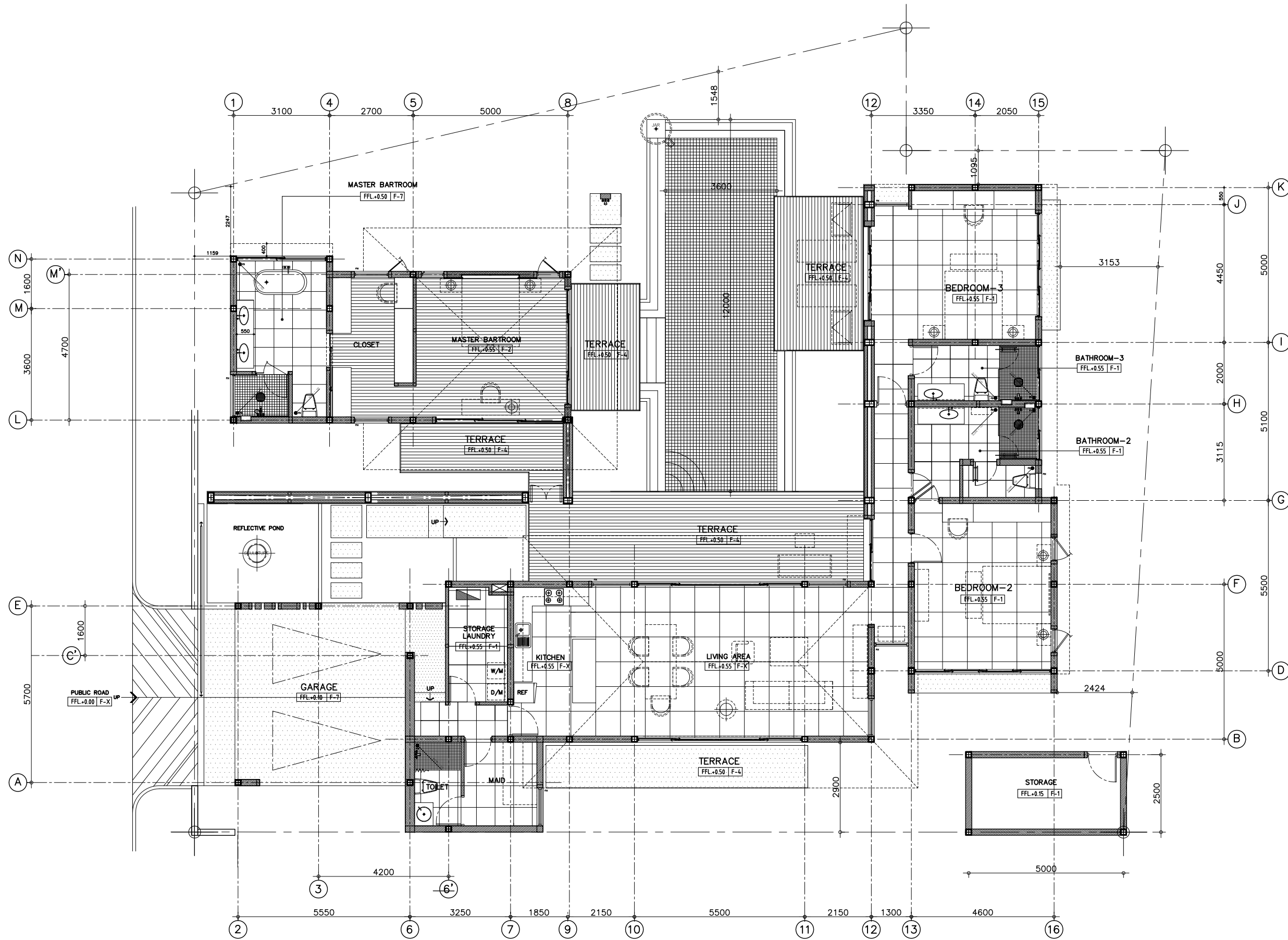
GROUND FLOOR PLAN P OT-
